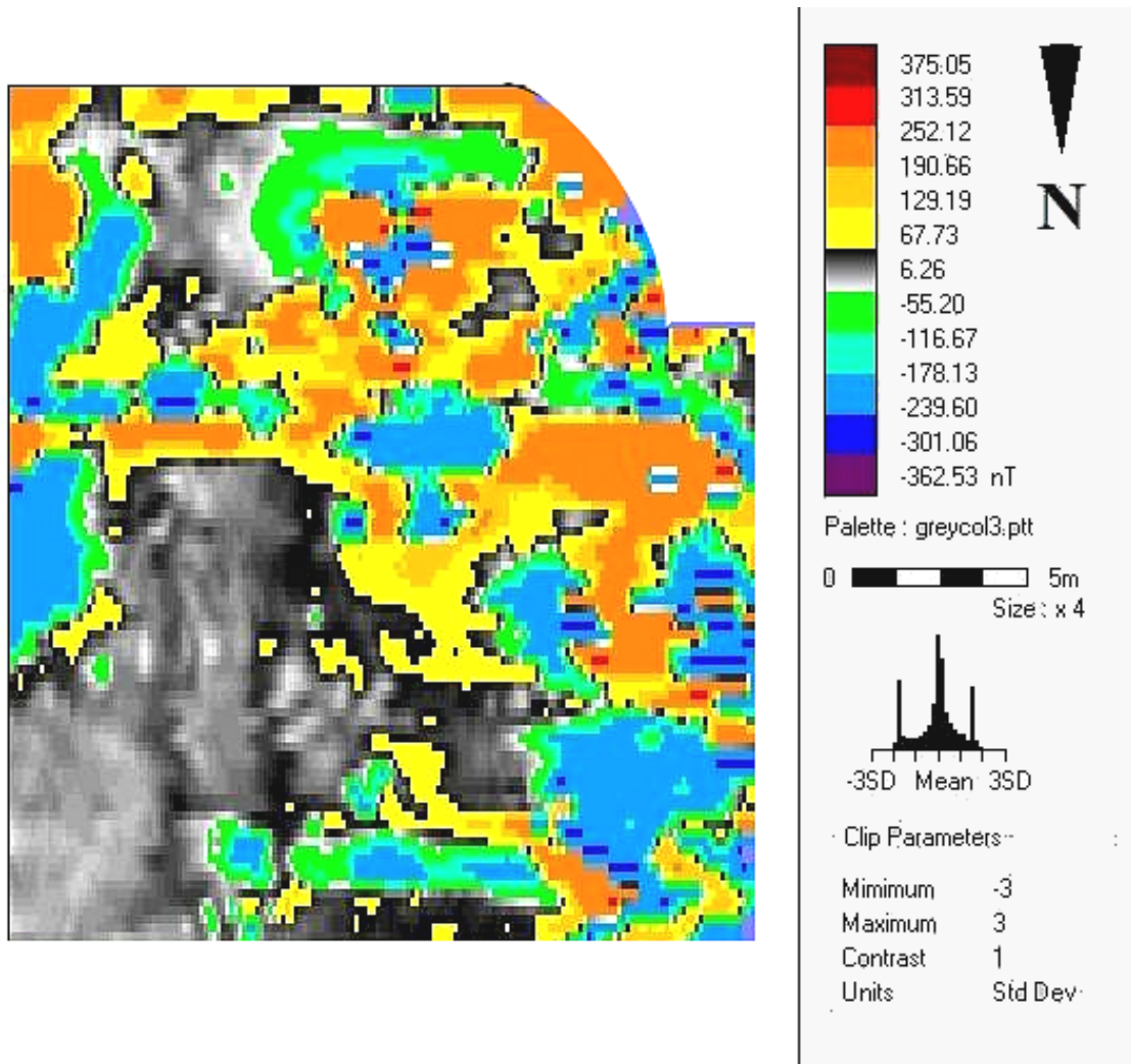
Figure S1 Magnetometer survey – Filtered results.
